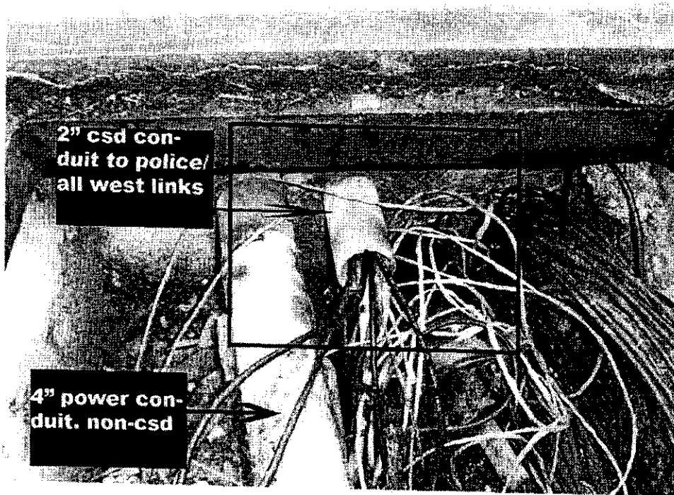
Figure 2 - Single 2" Duct - into Govt Admin Building - full.
